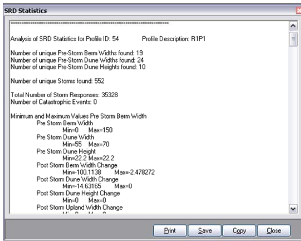
Figure 50. SRD statistics.
